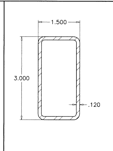
32 REINFORCING TUBE
