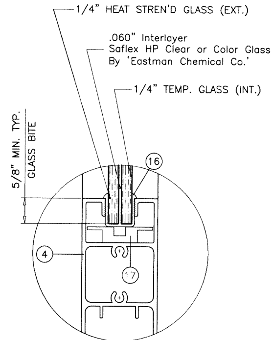
GLAZING DETAIL
