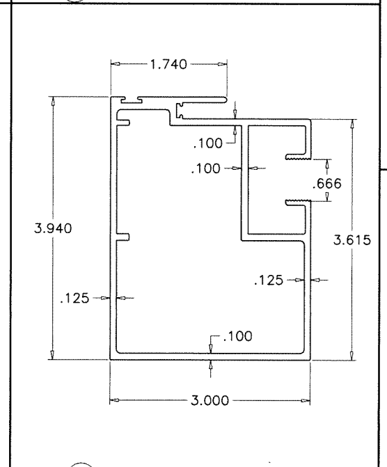
9 MAJOR INTERLOCK
