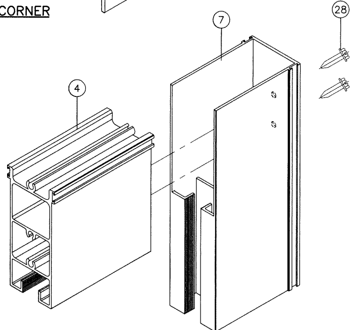
PANEL CORNER
