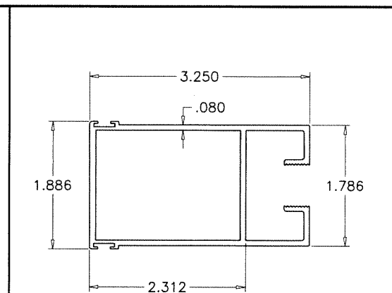
7 FIXED STILE
