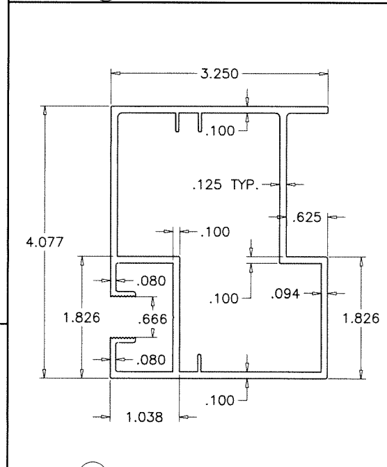
8 LOCKING STILE
